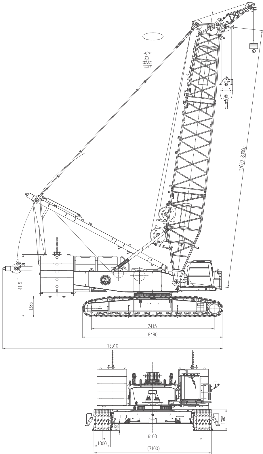
XLC200履带起重机外形图 XLC200 crawler crane outline dimension
