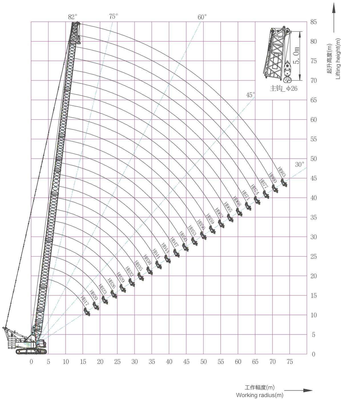
主臂工况_无臂端滑轮(HB/1)的主臂主钩工作范围图 Boom working condition _ boom main hook working range (without boom single top, HB/1)
